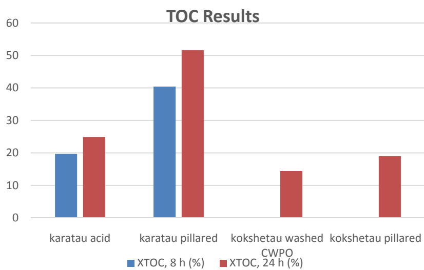
Figure 6 - Conversion of TOC in the removal of 4-nitrophenol by CWPO with natural and pillared clays from Karatau and Kokshetau catalysts at 8 and 24 hours of reaction time.
