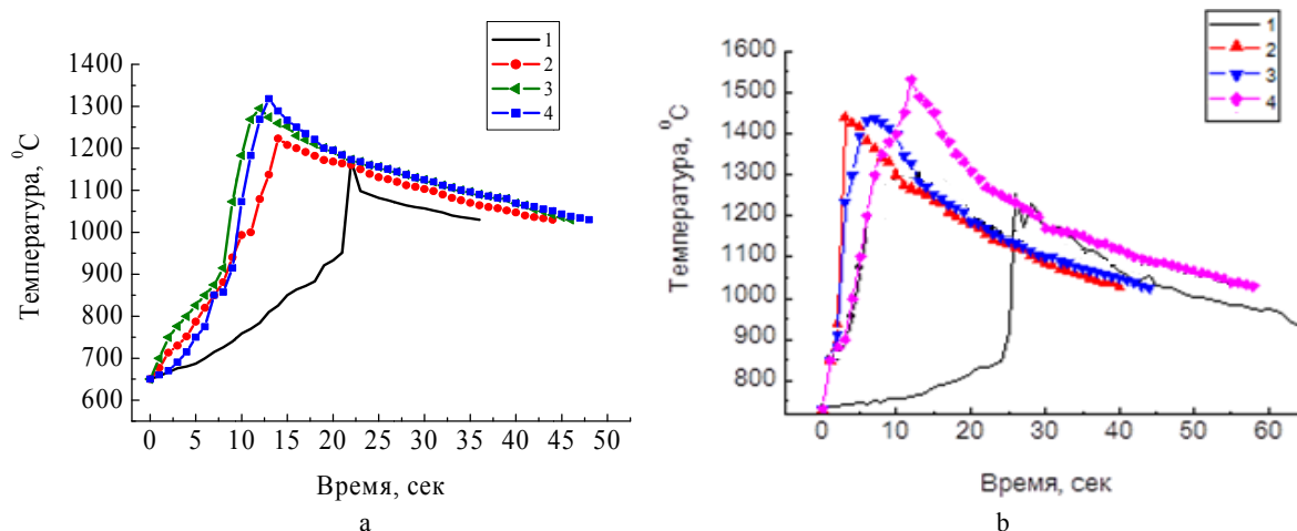
Figure 6 - Thermograms of combustion of the system ( \text{SiO}_2 + \text{Me} ) with aluminum and magnesium in the initial state and after 20 minutes of MCT with different amounts of graphite: a- \text{SiO}_2 + (\text{Al/C}) , b- \text{SiO}_2 + (\text{Mg/C}) ; 1 - Me initial; 2 - 5%; 3 - 10%; 4 - 20% C
