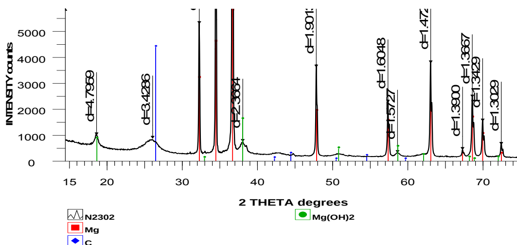
Figure 3- Diffraction of the sample (Mg 80% + C 20%), after 20 minutes of MCT
